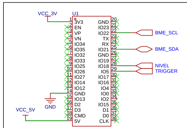
ESP32-DevKitC
